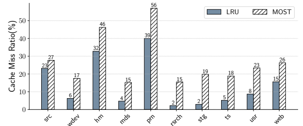
Figure 5. The MOST scheme causes more cache misses.
