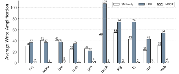
Figure 3. Average write amplification ratios of SMR-only and different cache algorithms under Microsoft traces.
