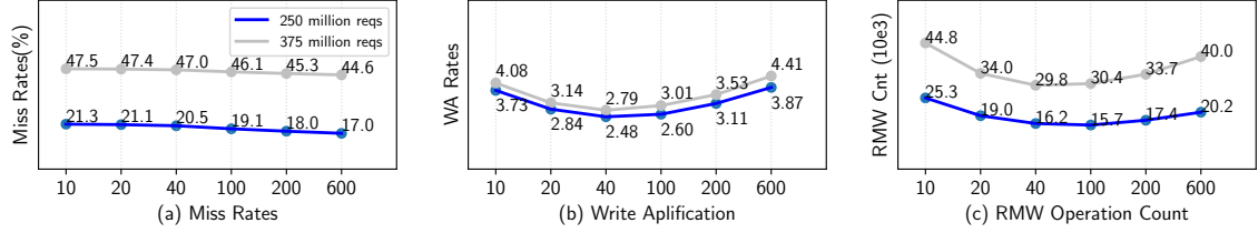
Figure 17. Impacts of different alternative band sizes ranging from 2MB to 600MB.
