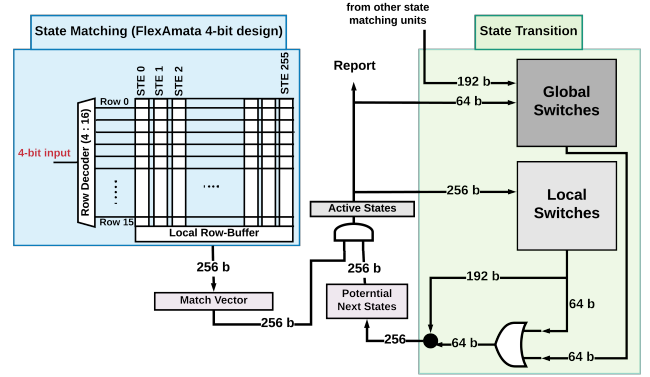
Figure 8. A 4-bit automata processing unit (4-bit CA-RDB).
