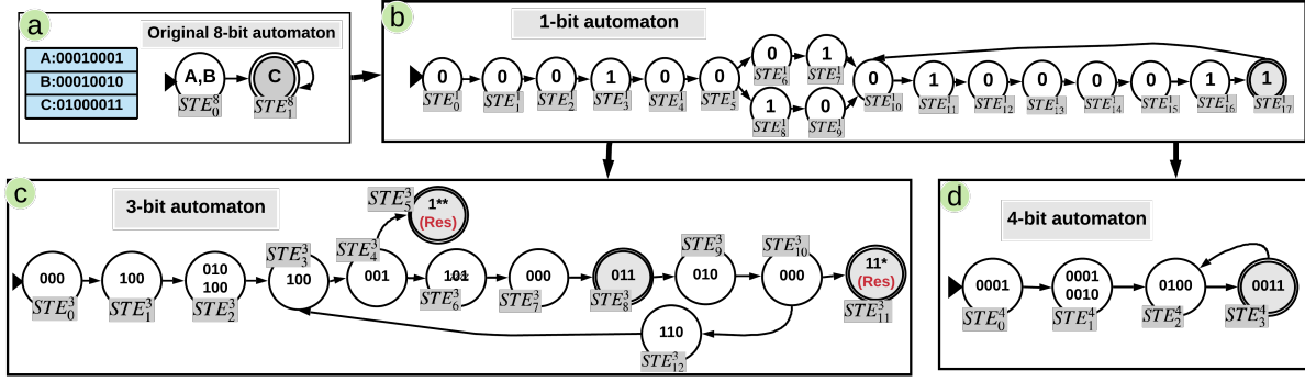
Figure 2. An 8-bit automaton (a) is converted to the minimized 1-bit automaton (b). The 3-bit (c) and 4-bit (d) automata are generated from the 1-bit automaton.
