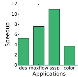
Figure 14. Performance advantage of using application-specific PEs over RISC-V soft-cores.
