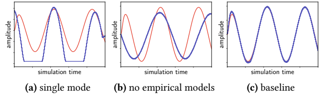
Figure 25. Effect of modes/empirical models on accuracy
