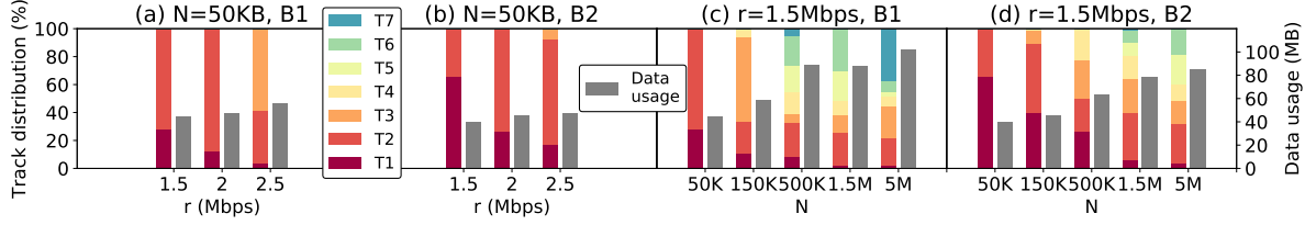
Figure 10. The track distribution and data usage for Hulu with different shaping policy and network conditions.
