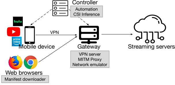
Figure 6. The system architecture of CSI
