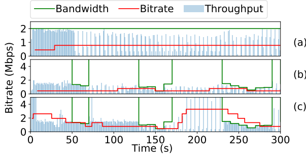
Figure 11. Hulu behavior under (a) 2Mbps, (b) profile B2, r=1.5\text{Mbps} , N=50\text{KB} , (c) profile B2, r=1.5\text{Mbps} , N=5\text{MB} .
