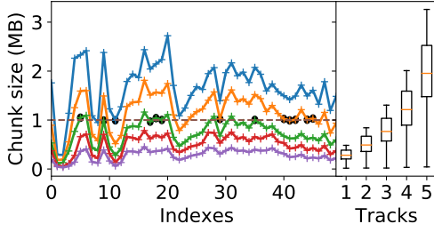
Figure 4. Chunk sizes of a Youtube video (PASR 2.6).
