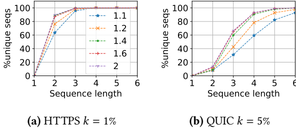
Figure 5. Relation between chunk sequence length and percentage of unique sequences for videos with different PSNR. Each line represents results for a PSNR.
