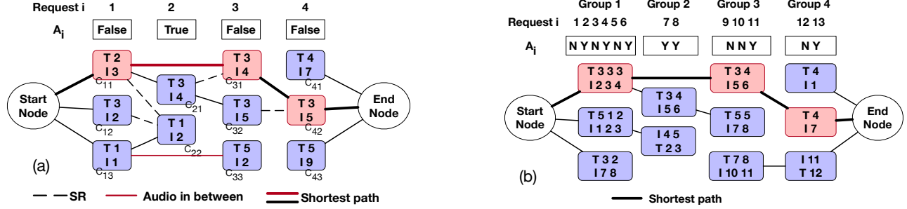
Figure 9. Sample graph for CSI inferencing: (a) For 3 types without transport multiplexing. (b) For type SQ. T stands for track, I stands for index.
