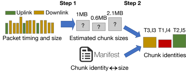
Figure 3. Proposed analysis approach for encrypted traffic (T: track, I: index, Tx,Iy means the y^{th} chunk in the x^{th} track.)
