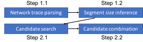
Figure 7. Algorithm overview
