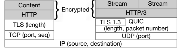
Figure 2. HTTPS/QUIC network stack (and available information)
