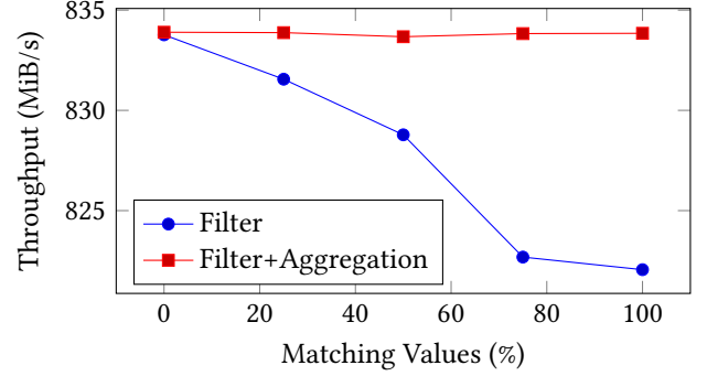
Figure 7. Throughput measurements for filtering and aggregating 1 GiB of NVMe data on the FPGA.
