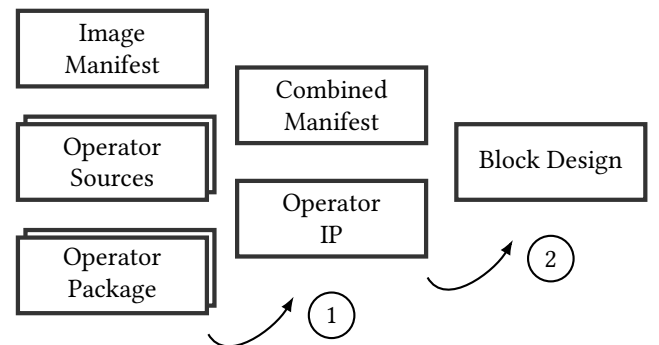
Figure 5. Inputs and artifacts in the Metal FS overlay build process. (1) Local operator sources and packages from npm are assembled into Vivado IP. (2) Together with a combined image manifest, the overlay Block Design is generated.
