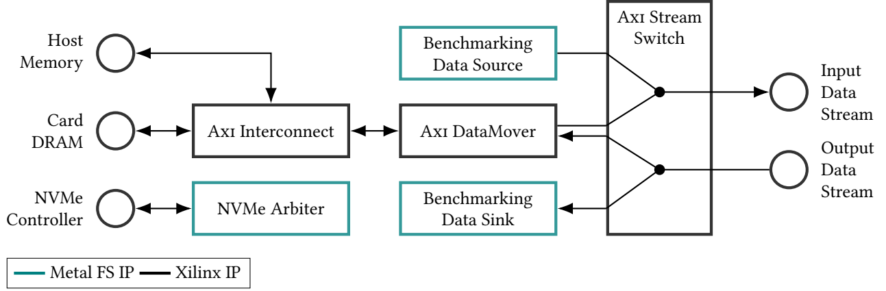
Figure 4. Flow of data in the Metal FS I/O subsystem. Host memory and DRAM are mapped at different offsets in the AXI Crossbar address space. Before starting a processing pipeline, the Data Selector AXI Stream Switch is configured to choose the data sources and sinks to be connected to the overlay stream switch.
