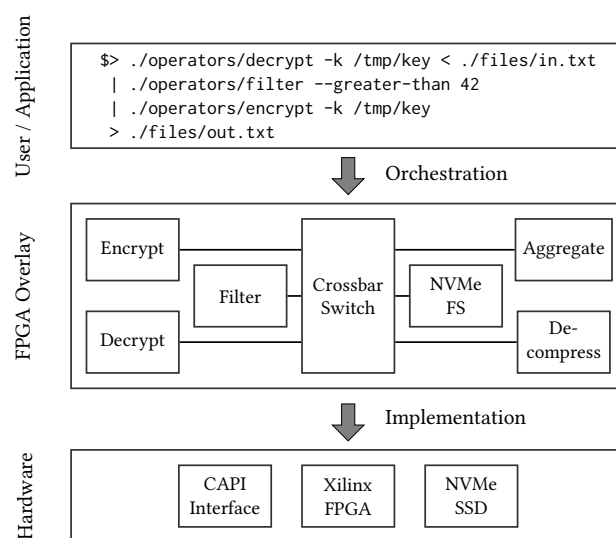
Figure 1. Shell commands issued by a user or application are executed by orchestrating a pipeline of pre-defined functional elements of a coarse-grained FPGA overlay. The overlay can be generated for most CAPI-enabled FPGAs.
