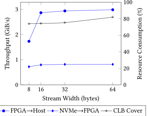
Figure 6. Throughput and resource consumption of overlay images with different stream widths. All images contain three placeholder operators. Throughput was measured with a 1 GiB data transfer. The translation of file offsets into physical blocks is part of the NVMe measurements.
