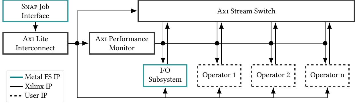
Figure 3. Internal structure of the FPGA overlay design. The SNAP Job Interface receives configuration data from the host and configures the corresponding system components through an interconnect bus. A performance monitor observes the transactions on the stream interfaces.
