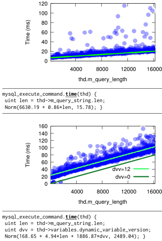
Figure 5. mysql_execute_command , 5.7.24 (top) vs. 8.0.11.
