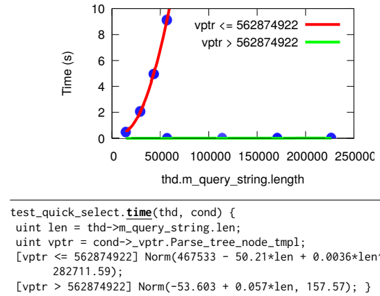
Figure 6. test_quick_select() : IN vs AND/OR query.
