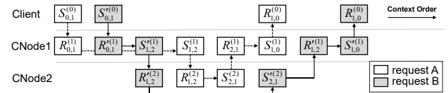
Figure 5. IntraServpod causality: request B is issued earlier by Servpod1, but returned later than request A.
