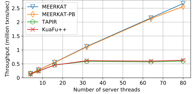
Figure 5: Peak throughputs comparison between Meerkat and the three other systems for uniform key access distribution for Retwis transactions. The comparison systems are able to scale better with coordination due to Retwis’s longer transactions and read-heavy workload. However, none of the systems quite scale linearly to 80 cores except Meerkat; the non-ZCP systems continue to be limited by their additional coordination.
