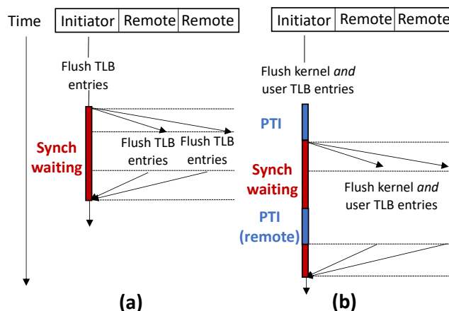
Figure 1. (a) In the baseline Linux TLB shootdown protocol, much of the shootdown is spent synchronously waiting for remote flushes. (b) Kernel page table isolation (PTI), a mitigation for Meltdown, exacerbates this wait time.
