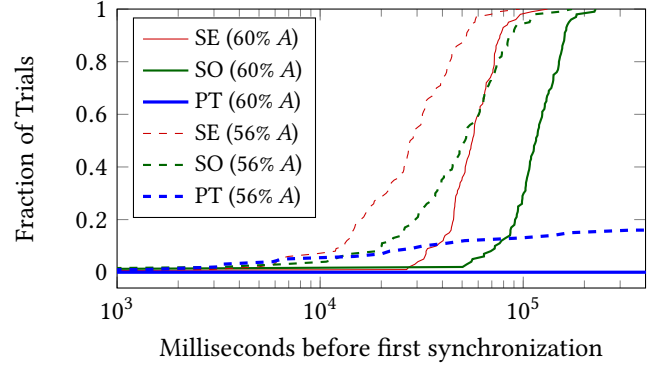
Figure 8. CDF of time until first synchronization under the three strategies static equal (SE), static optimal (SO), and predictive treaties (PT), for slack allocation with varying bias at the first station. Stations received 100 votes per second.
