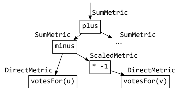
Figure 6. Metrics tree created by example code
