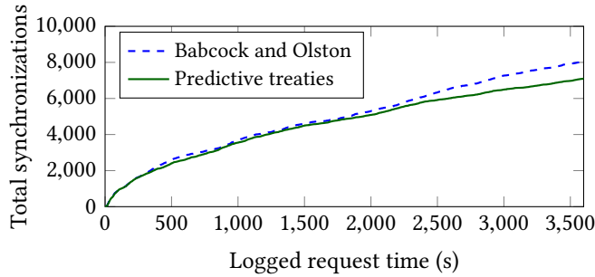
Figure 12. Using synchronizations to compare Babcock and Olston’s top- k algorithm with using predictive treaties.
