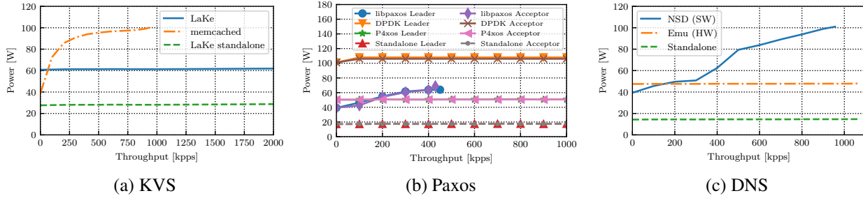
Figure 3. Power vs throughput comparison of KVS (a), Paxos (b), and DNS (c). in-network computing becomes power efficient once query rate exceeds 80Kppsm 150Kpps and 150Kpps, respectively
