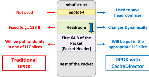
Figure 10. CacheDirector changes to the mbuf structure.
