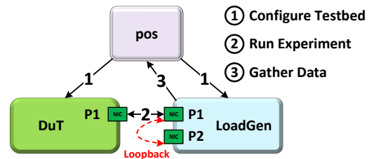
Figure 11. Experiment setup.
