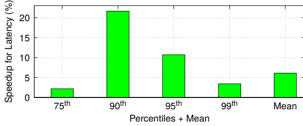
Figure 1. Speedup achieved for a stateful service chain (Router-NAPT-LB) at high-percentiles and mean by using CacheDirector while running at 100 Gbps.
