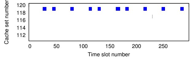
Figure 4. Unmitigated concurrent LLC side-channel attack on x86. The pattern at set 119 shows the victim’s cache footprint detected by the spy.
