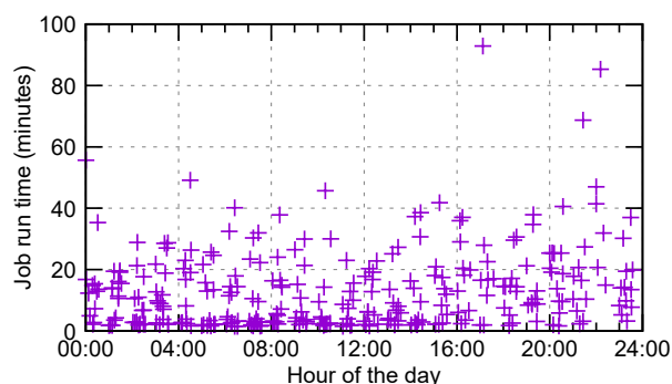
Figure 1. Run times of 300 copy jobs over 2 weeks. All days are overlaid over their 24 hours.
