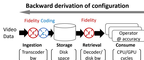
Figure 1. The VStore architecture, showing the video data path and backward derivation of configuration.
