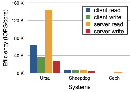
Figure 7. IOPS efficiency.
