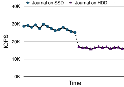
Figure 11. Journal expansion.
