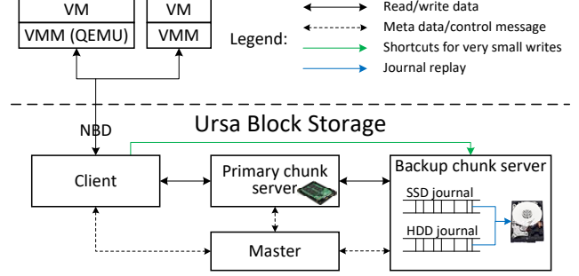
Figure 3. Ursa architecture. Clients are a portal providing the block interface to VMMs (virtual machine monitors).
