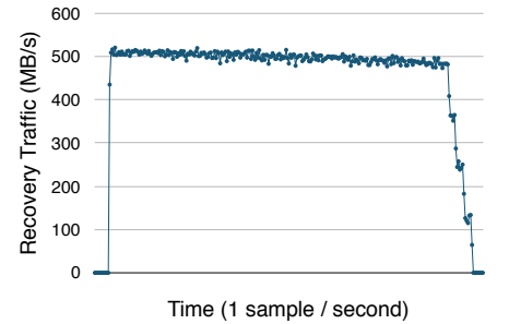
Figure 12. Failure recovery.
