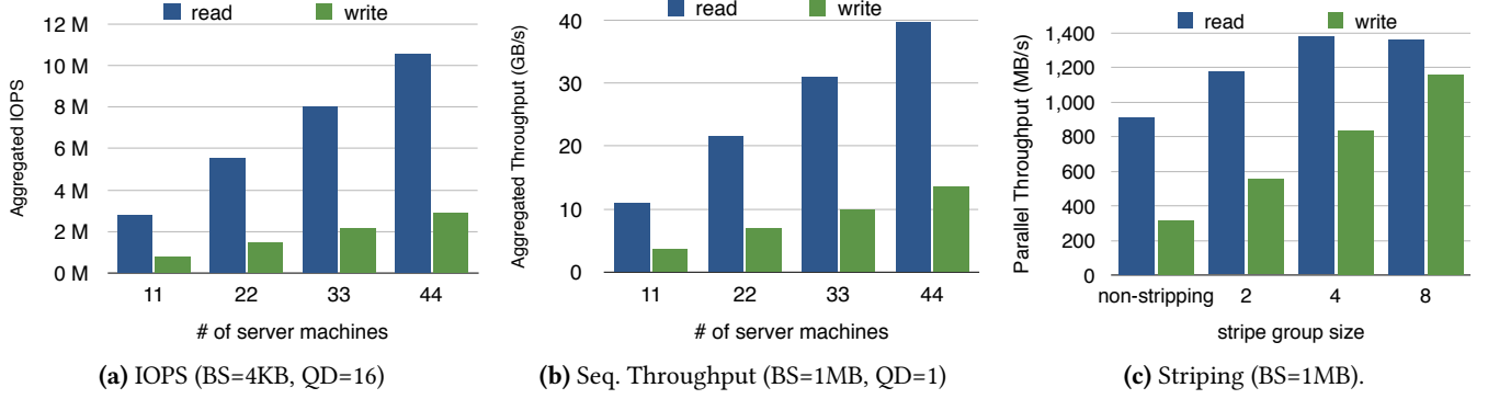
Figure 13. Scalability test.
