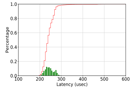
Figure 16. Latency PDF &amp; CDF.
