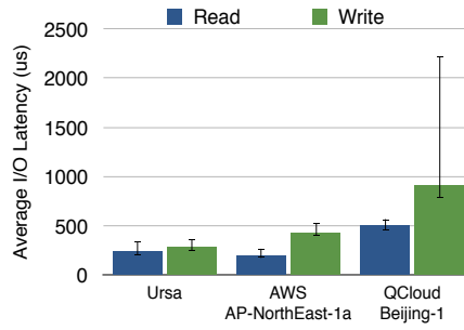
Figure 15. Public cloud latency.
