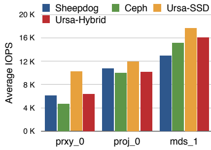
Figure 14. Trace-driven comparison.
