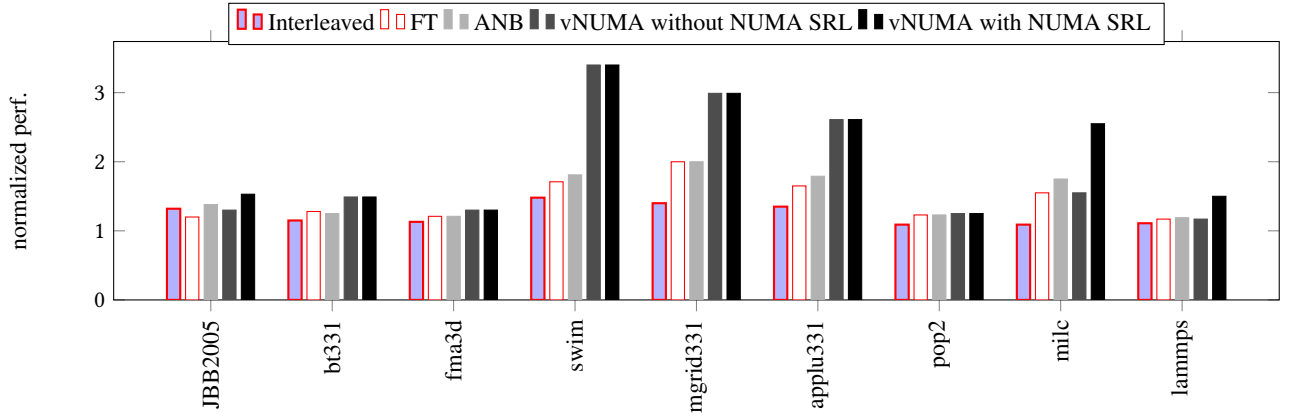
Figure 7. vNUMA compared with the state-of-the-art blackbox solutions (higher is better). This experiment also highlight the importance of NUMA policies embedded within the SRL. No topology change is triggered during this experiment.
