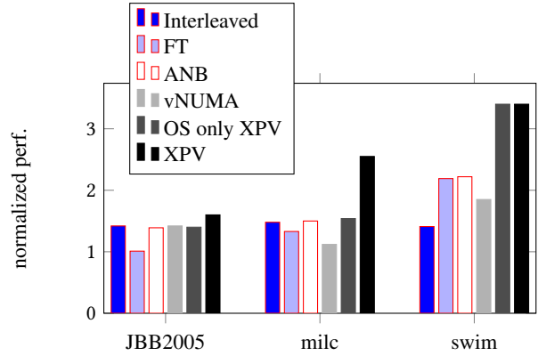
Figure 9. XPV facing vCPU loadbalancing due to the overcommitment of the CPU resource (higher is better).
