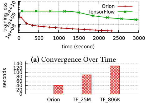
Figure 13. Orion vs. TensorFlow, SGD MF on Netflix
