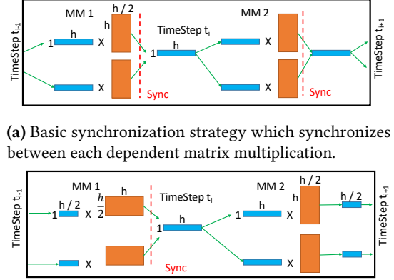
(a) Basic synchronization strategy which synchronizes between each dependent matrix multiplication. (b) Single synchronization strategy that precomputes partial sums and uses reduction to eliminate a synchronization.
