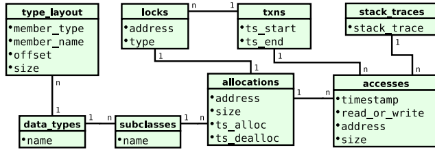
Figure 6. LockDoc database schema storing the recorded trace in a structured form, revolving around the central memory accesses table.
