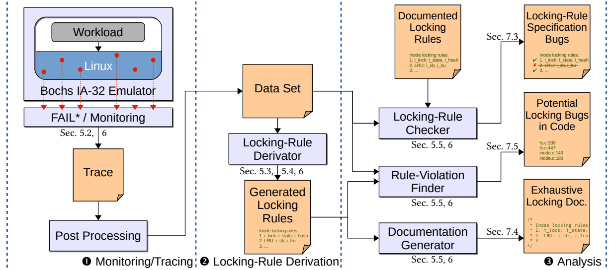
Figure 5. LockDoc overview: Based on a memory-access and lock acquisition trace from the Linux kernel (phase ❶), we infer the most probable locking rules for a specific set of data structures (❷). Using this information, we look for locking-rule documentation bugs, locking bugs in the code, and generate exhaustive locking documentation (❸).
