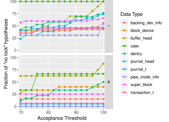
Figure 7. Fraction of “no lock” locking-rule hypotheses for different acceptance thresholds t_{ac} , separately plotted for each observed data type and read vs. write accesses.
