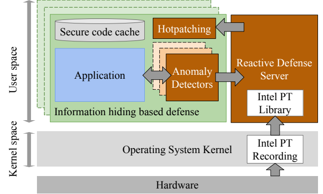
Figure 2. ProbeGuard architecture
