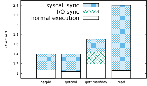
Figure 4. Microbenchmarks. Relative performance overhead of a selected number of syscalls. For the read syscall we read a 512 KB file.
