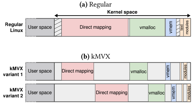
Figure 3. Regular kernel virtual address space, and the kMVX partitioned non-overlapping address space.
