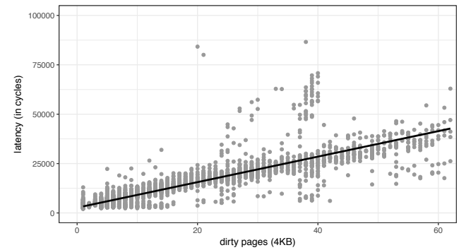
Figure 12. Scatter-plot of revert cost vs. change set size. Black line shows linear regression. Mean revert cost is approximately 11,000 cycles.
