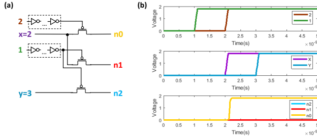
Figure 8. SPICE simulation results, using a 180nm CMOS library, for a RaceTree implemented with single transistor INHIBITs. To reduce the overhead of the chains of inverters, required for the delay of inhibiting inputs (to avoid glitches in case both i and j arrive at the cycle), rather than embedding them in each INHIBIT we place them at the threshold lines and share them between various cells.
