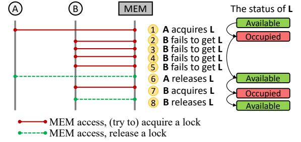
Figure 2. A spin lock based on shared memory.
