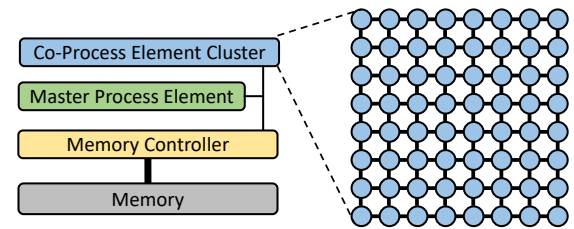
Figure 1. The architecture of SW26010.
