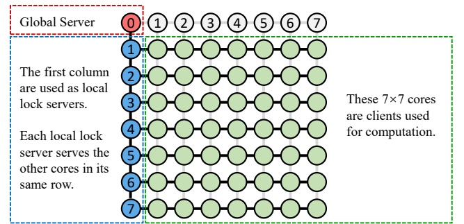
Figure 9. Mapping the cores to global lock server, local lock servers and clients.
