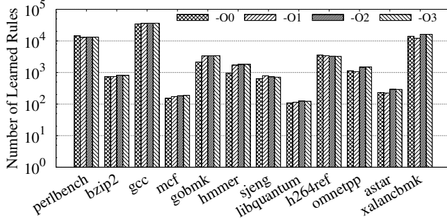
Figure 6. Sensitivity of learning on optimization levels.
