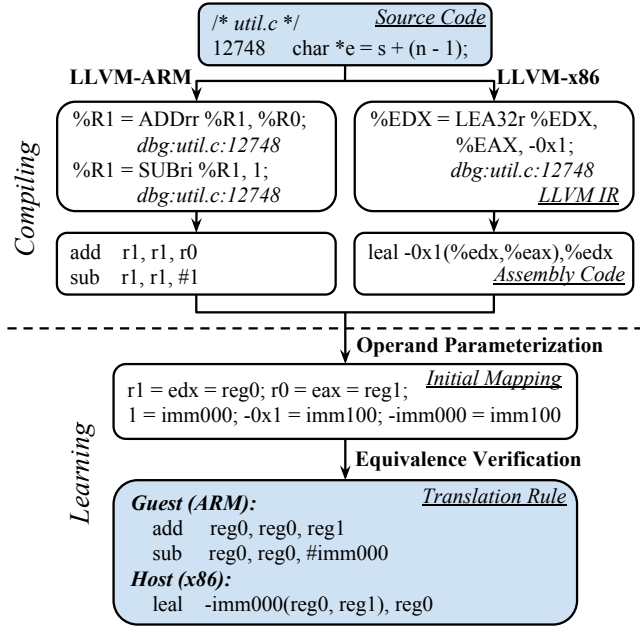
Figure 1. The learning process of translation rules.
