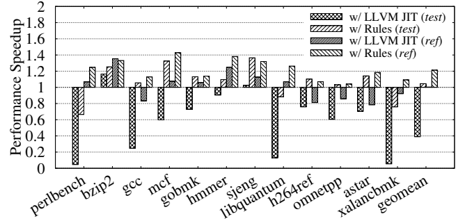
Figure 9. Performance speedup for guest GCC binaries.
