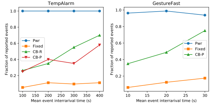
Figure 10. Sensitivity of accuracy to event inter-arrival.
