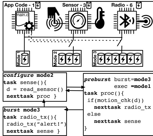
Figure 5. Overview of Cappybara. The platform has resources for computation, sensing, and communication, and includes three energy storage configurations with different capacities. An example program has tasks annotated with energy mode requirements.
