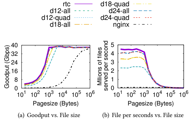
Figure 6. DLibOS and RTC webserver performance compared to NGINX using various layout configurations and different file sizes.
