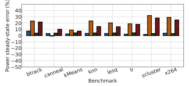
(b) Power steady-state error in Phase 1.
