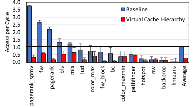
Figure 8. Bandwidth reduction of IOMMU TLB.
