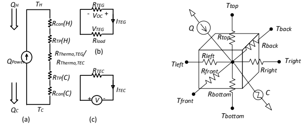
Figure 2 (a) Thermal circuit model of thermocouple elements. (b) Electric circuit model of TEGs. (c) Electric circuit model of TECs.
