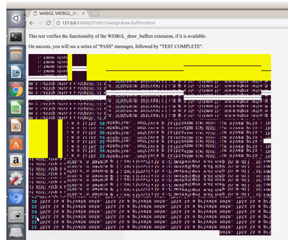
Figure 2. Exploiting vulnerability #10 in Table 1. The exploit manages to access to unauthorized parts of the GPU memory, which holds previously rendered UI content. In this snapshot, the exploit has accessed the content of a text previously edited in a native text editor.
