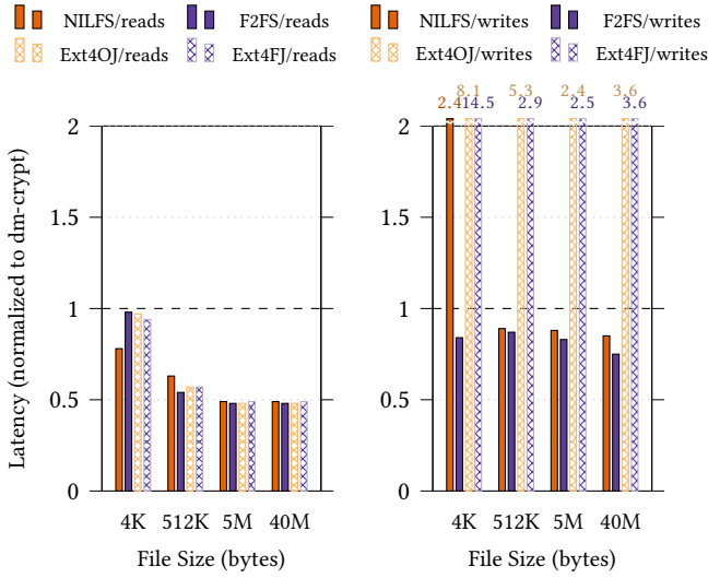
Figure 5.a: Sequential reads.
