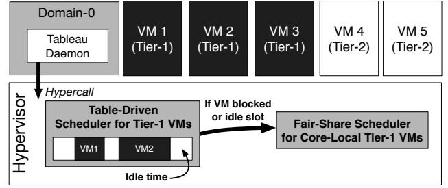
Figure 1: Tableau architecture
