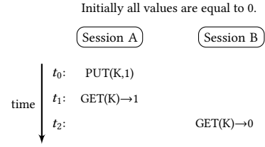
Figure 5: Session B seeing the old value is a violation of Lin, but not SC.
