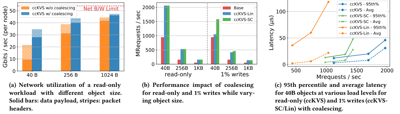
Figure 13: Analysis of coalescing and latency. [9 nodes, \alpha = 0.99 ]
