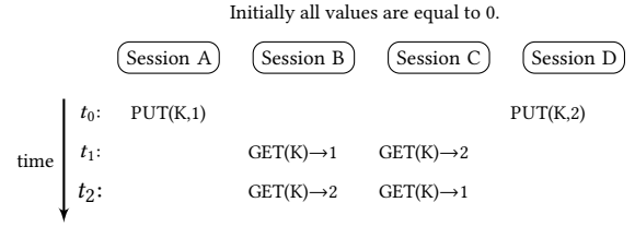
Figure 6: Sessions B and C do not agree on the order of writes and hence this is a SC violation (also a Lin violation).
