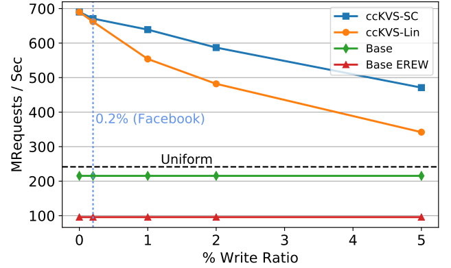
Figure 10: Sensitivity to write ratio. [9 nodes, \alpha = 0.99 ]
