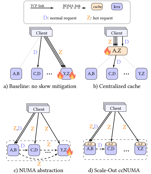
Figure 2: Design space for skew mitigation techniques.
