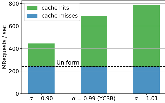
Figure 9: Break-down of completed requests in ccKVS for a read-only workload with varying skew. [9 nodes]
