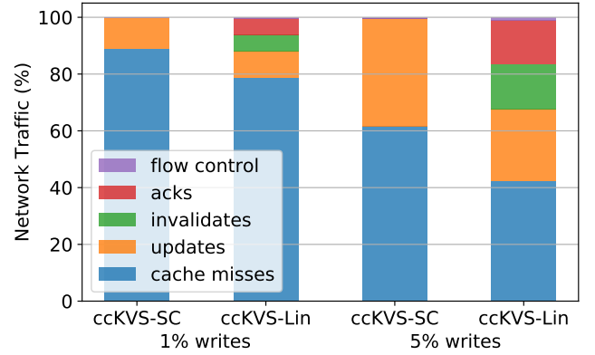
Figure 11: Network traffic breakdown. [9 nodes, \alpha = 0.99 ]
