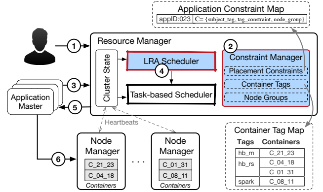
Figure 6: MEDEA architecture
