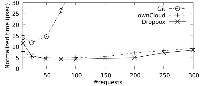
Figure 6: Normalized invariant checking and trimming time
