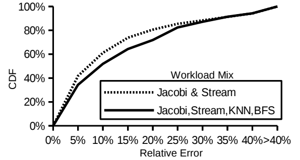
Fig. 9: The cumulative distributions of prediction error for two distinct mixed workloads.
