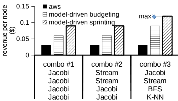
Fig. 13: Dollars earned for a burstable instances which optimizes the sprinting policy based on budget and timeout.
