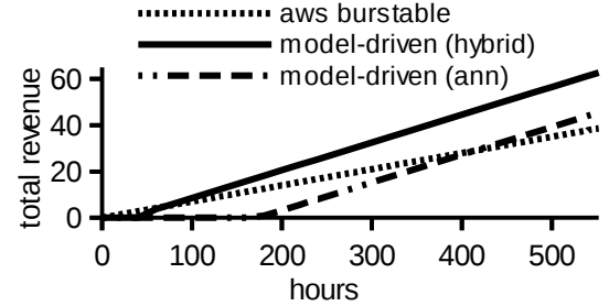
Fig. 14: The number of hours required to offset the profiling cost using our model.
