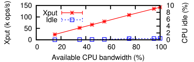
Figure 10: Throughput of Redis YCSB workload A and idle time vs available bandwidth.
