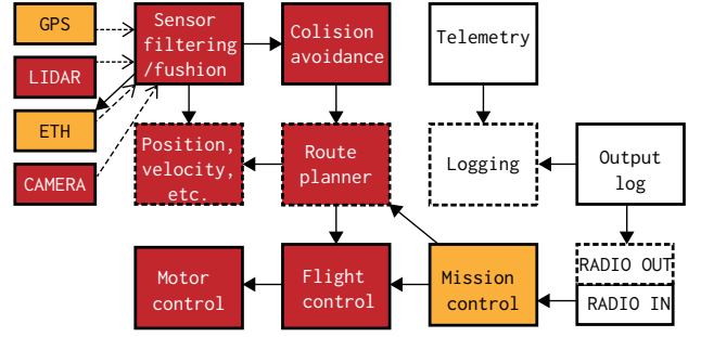
Figure 2: Simplified AAV design, showing main components (seL4 address spaces). Solid frames indicate active components, broken frames passive ones. Solid arrows indicate RPC-style server invocation, dashed arrows are completion signals. For clarity we do not show most invocations of the logging service, this would add a solid arrow from each component to the "Logging" box. Most critical components are shown in red, least-critical ones in white.
