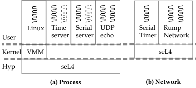
Figure 8: Architecture of isolation benchmarks.
