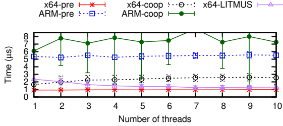
Figure 14: Execution time of seL4 user-mode EDF scheduler compared to kernel scheduler in x64 LITMUS RT .
