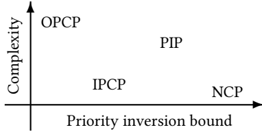
Figure 1: Comparison of RT locking protocols based on implementation complexity and priority inversion bound.
