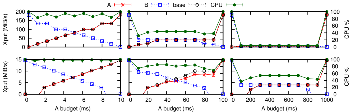
Figure 11: Throughput for clients A and B of a passive AES server processing 10 requests of 4 MiB of data with limited budgets on the x64 (top row) and ARM (bottom row) platforms. The two clients’ budgets add up to the period, which is varied between graphs (10, 100, 1000 ms). Clients sleep when they process each 4 MiB, until the next period, except when their budgets are full. Each data point is the average of 10 runs, error bars show the standard deviation.
