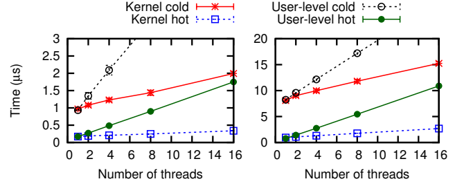
Figure 13: Cost of switching the priority of n threads in kernel and user level, with hot and cold caches, on Haswell (left) and Sabre (right). All data points are the average of 100 runs, with very small standard deviations.
