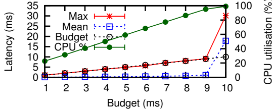
Figure 9: Average and maximum latency of UDP packets with a high-priority CPU hog running with a 10 ms budget.
