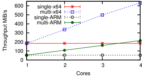
Figure 12: Results of the AES shared-server multicore case study on Sabre and Haswell. Single shows results for a passive server thread migrating between cores to service clients while multi has one passive thread per core. For both series, the number of clients is equal to the number of cores and each client requests 1MiB of data encrypted.
