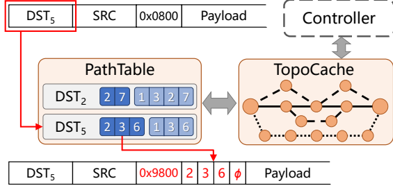
Figure 4: Host cache.
