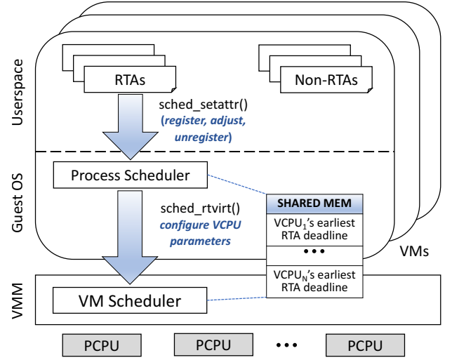
Figure 2: Overview of the architecture of RTVirt. RTAs register, adjust parameters, and unregister with their OS in the VM using an existing system call. The guest OS communicates the VM's scheduling parameters with the VMM on the host using a new hypercall and shared memory. The two levels of schedulers work cooperatively to enforce timeliness guarantees for the virtualized RTAs.
