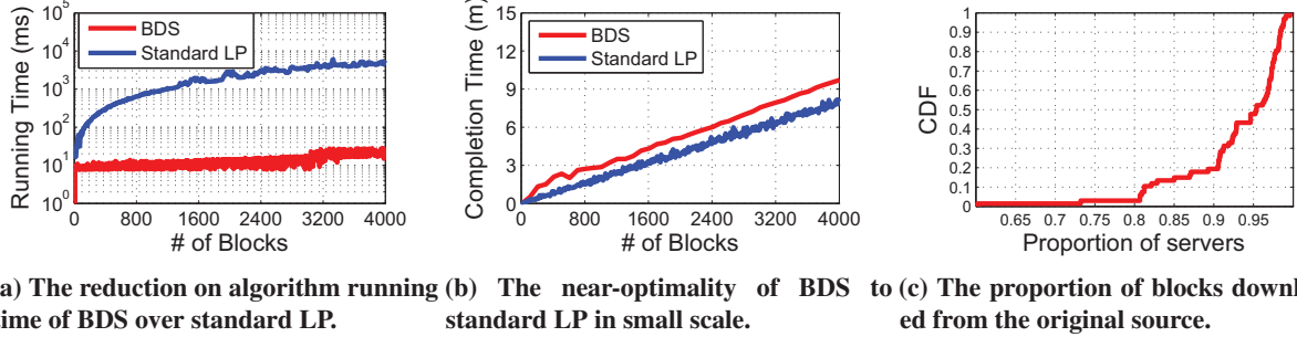
Figure 13: [In-depth analysis] on (a) reduction on algorithm running time, (b) near-optimality, and (c) effects of overlay transmission.
