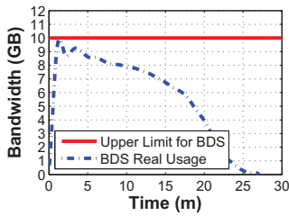
Figure 10: The effectiveness of bandwidth separation.
