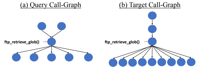
Figure 5. The call-graphs surrounding Wget 's ftp\_retrieve\_glob() procedure in the MIPS query (left) and a target from a NETGEAR firmware (right). The variance in call-graph structure prevents graph based techniques (e.g., BinDiff ) from succeeding.
