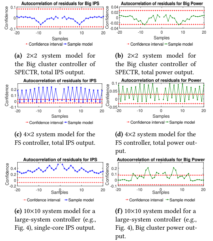
Figure 15. Autocorrelation of residuals for identified system models of different sized MIMO controllers. We show a single performance and power output for each modeled system across multiple inputs.
