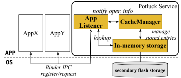
Figure 4. System architecture.
