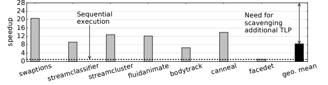
Figure 3. Highest speedup obtained by nondeterministic PARSEC benchmarks on a 28 cores Intel-based platform.
