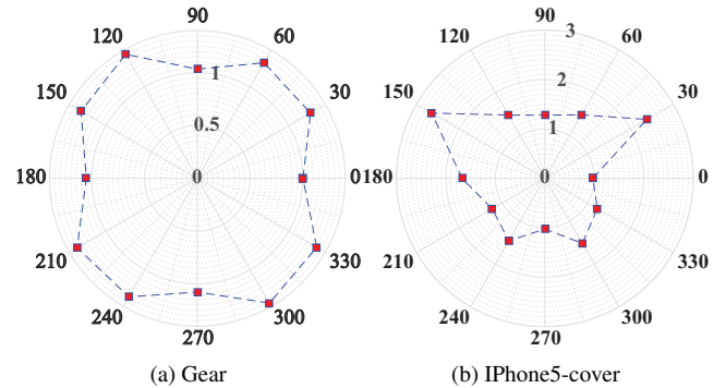
Figure 14: Energy consumption with power-gating strategy under different orientations. The markers represent the normalized energy consumption.
