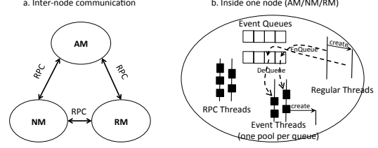
Figure 4. Concurrency and communication in MapReduce (a vertical line: a thread; a black rectangle: a RPC function or an event handler)
