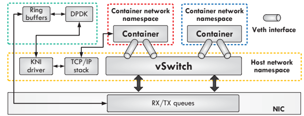
Figure 2. DDPK enabled container networking.
